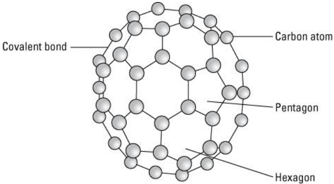
This is C60 also called a buckyball.
