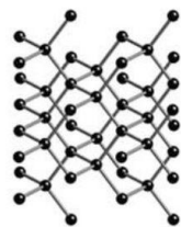
Diamond
