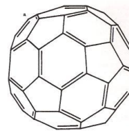
C 60 Buckyball
