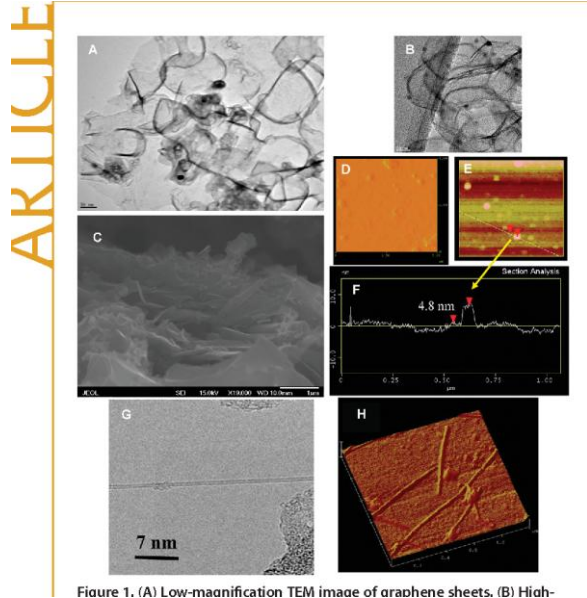
Figure 1. (A) Low-magnification TEM image of graphene sheets. (B) High magnification TEM image of few-layer graphene sheets overlaid side-by-side. (C) SEM image of the semitransparent graphene sheets synthesized in large quantities. (D) High-pass filtered AFM scan of graphene sheets overlaid on the Si surface. (E) AFM image of the few-layer graphene sheets, with (F) a corresponding AFM height image. (G) High-resolution TEM image of the single-wall carbon nanotubes used for this study. (H) AFM images of the nanotubes used for this study. The diameter of the nanotubes ranged from 0.8 to 1.2 nm.
