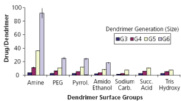
Figure 2. Encapsulation efficiency of indomethacin into STARBURST® dendrimers. Different dendrimer surfaces shown: primary amine, poly(ethylene glycol), carbomethoxypyrrolidinone, amidoethanol, sodium carboxylate, succinamic acid, and tris(hydroxymethyl)amidomethane.
